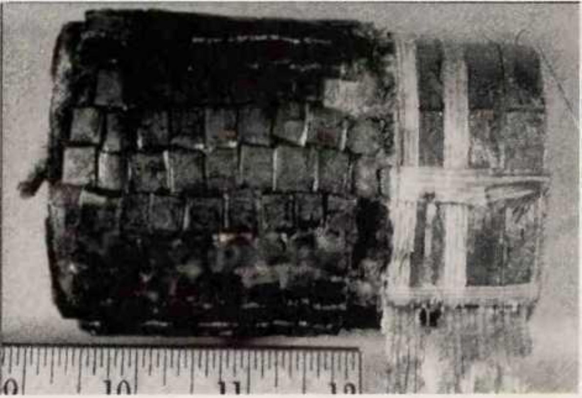
Close-up of the explosive charge of bomb #17. Note the shrapnel carefully glued to the bomb to increase its lethality. (FBI photograph)
