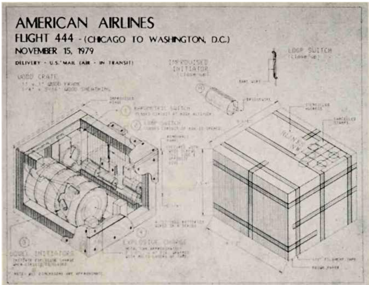
FBI diagram of bomb #3 that caused a fire on board American Airlines Flight 444 on November 15, 1979. Its unique and elaborate design— use of a barometer as altimeter, multiple triggering and booby-trap mechanisms— impressed federal explosives experts. (FBI photograph)
