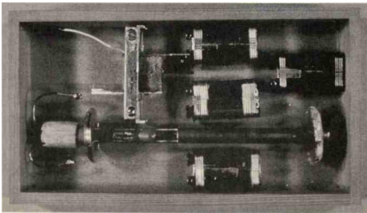
FBI Crime Laboratory's reconstruction of the bomb that nearly killed Yale professor David Gelernter on June 24, 1993. Kaczynski had finally found "the perfect detonator." (FBI photograph)
